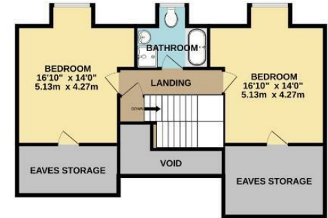
2ND FLOOR 773 sq.ft. (71.8 sq.m.) approx.
